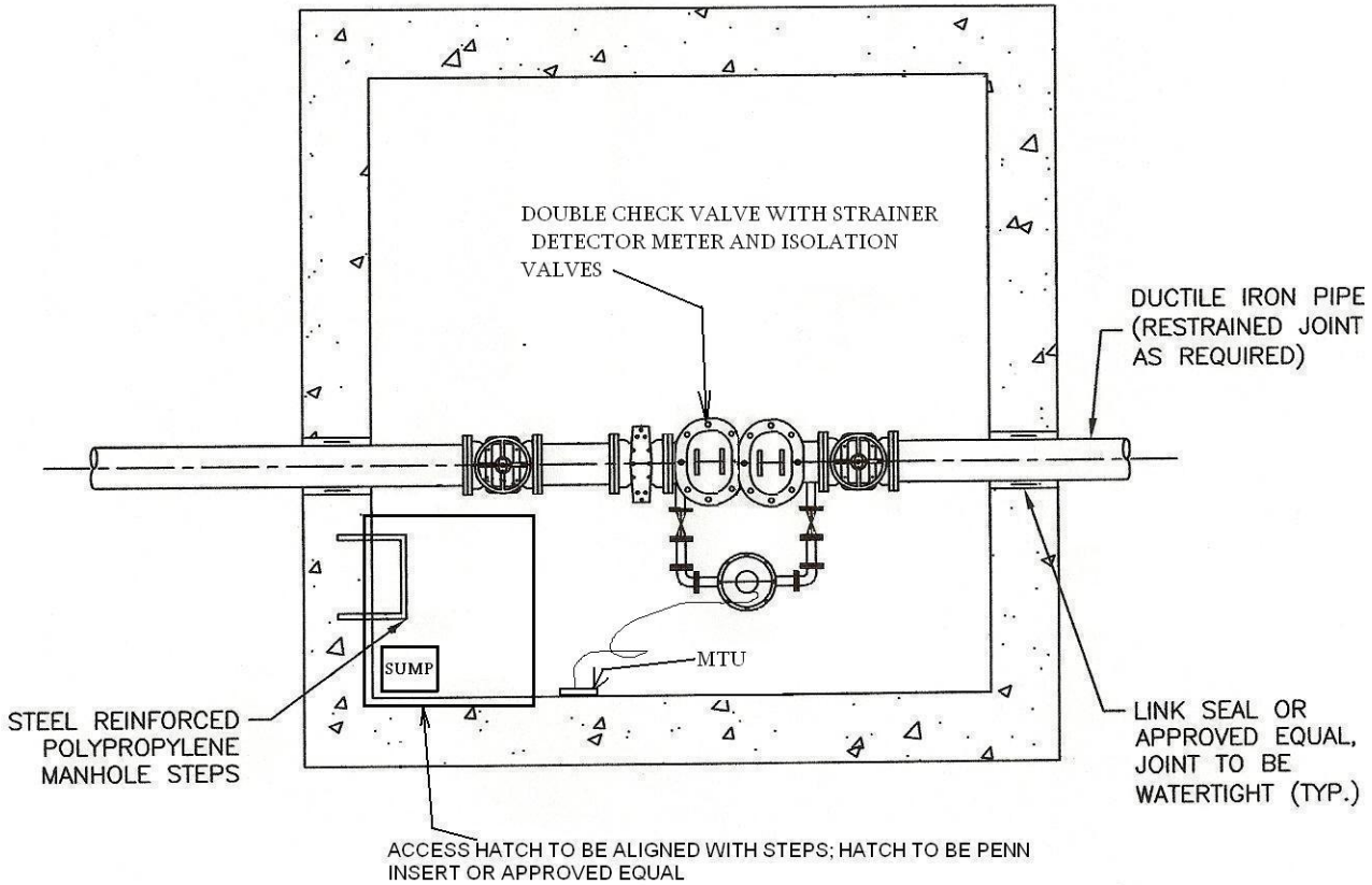
SECTIONAL PLAN (NOT TO SCALE)
