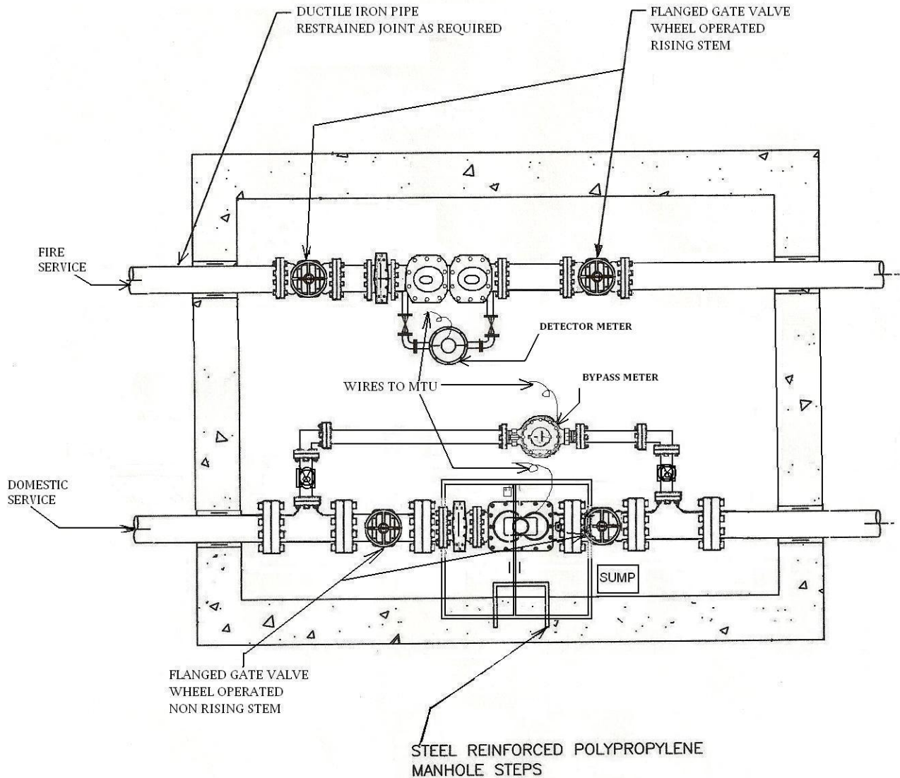
SECTIONAL PLAN (NOT TO SCALE)
