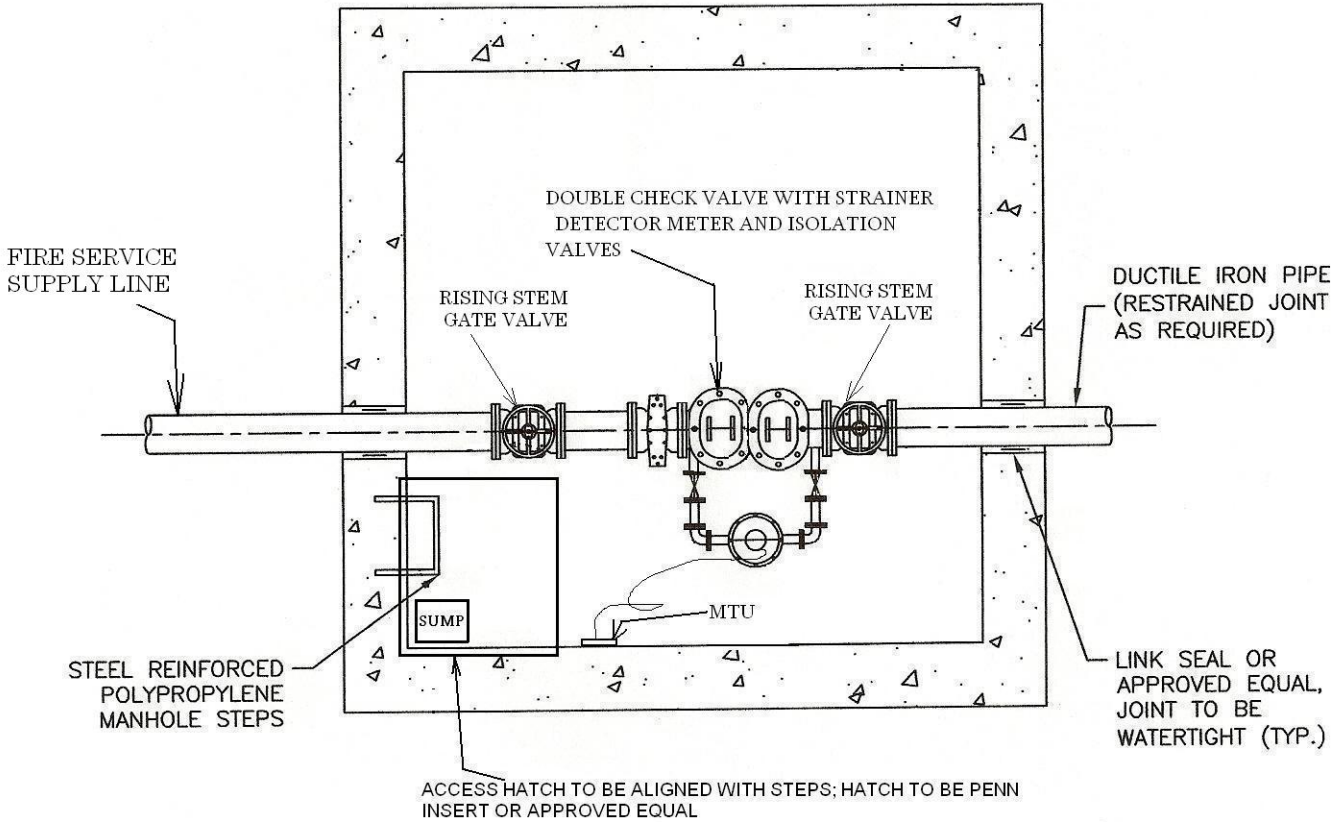
SECTIONAL PLAN (NOT TO SCALE)
